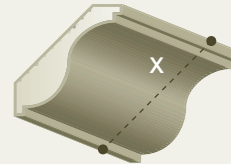
INT-506 x: 18.75cm x: 7-1/2"
