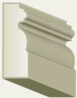
BA-404 ancho: 3.75cm (superior); 6.25cm (inferior) alto: 18.75cm
